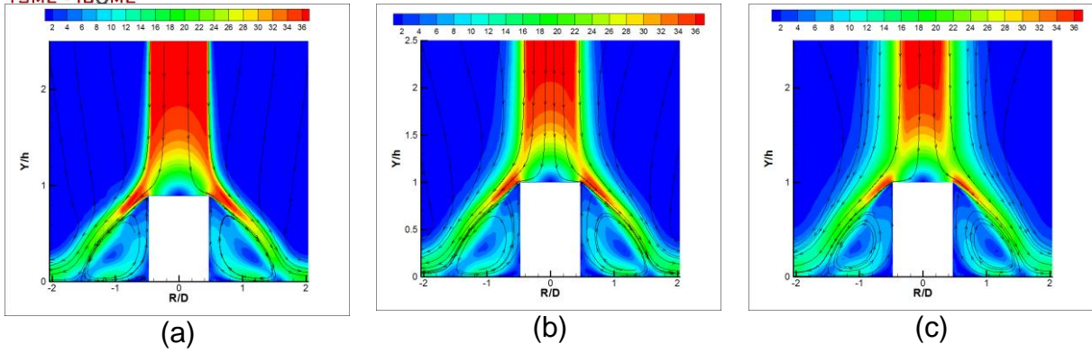
Fig. 3 Velocity contour around the pedestal ( v^2 - f , Re=23000 ) (a- H/D=2 , b- H/D=4 , c- H/D=6 )
