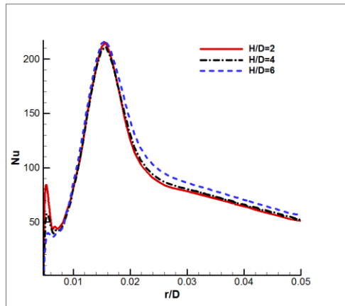
Fig. 12 Profiles of surface heat transfer coefficient along the flat plate ( v^2 - f , Re=50000 )
