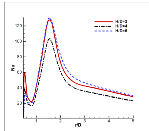
Fig. 11 Profiles of surface heat transfer coefficient along the flat plate ( v^2 - f , Re=23000 )
