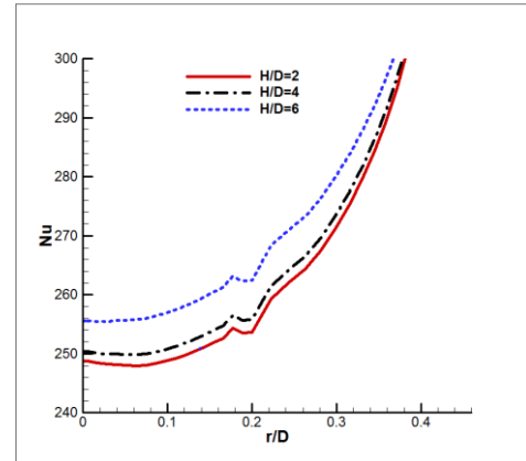
Fig. 10 Profiles of heat transfer coefficient along the pedestal top face ( v^2 - f , Re=23000 )
