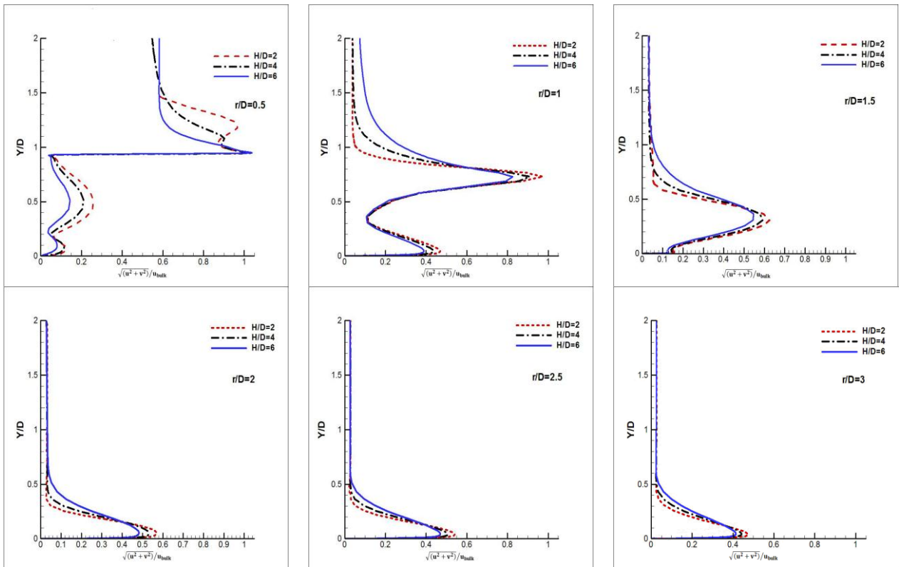
Fig. 5 Profiles of normalized velocity magnitude at different radial location ( v^2 - f , Re=23000 )
