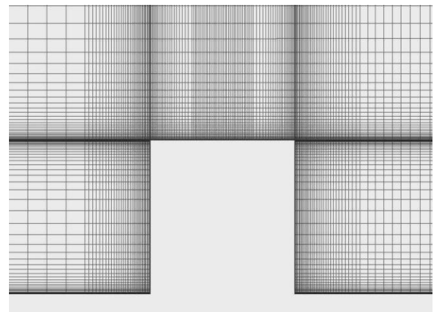
Fig. 2 The grids close to the pedestal
