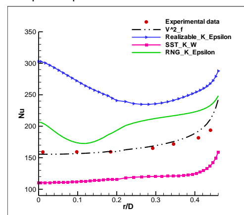
Fig. 7 Profiles of surface heat transfer coefficient along the pedestal top face ( H/D=6 , Re=23000 )
