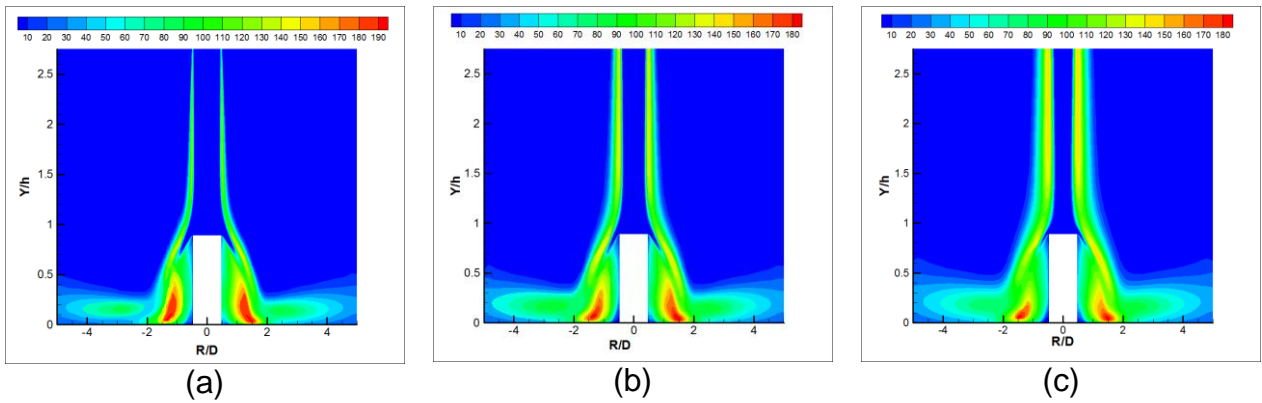
Fig. 4 Contour of turbulent kinetic energy around the pedestal ( v^2 - f , Re=50000 )
